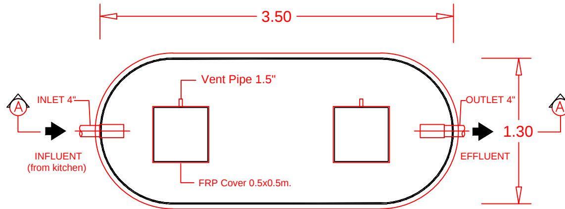
PLAN VIEW
