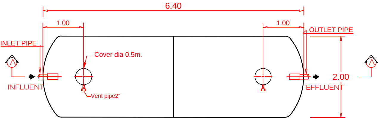
STAR TANK MODEL STD-2020
