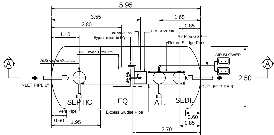
STAR SA-08500Z PLAN VIEW
