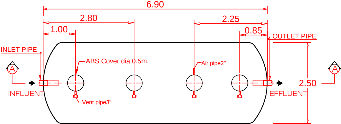
STAR TANK MODEL STD-2534A
