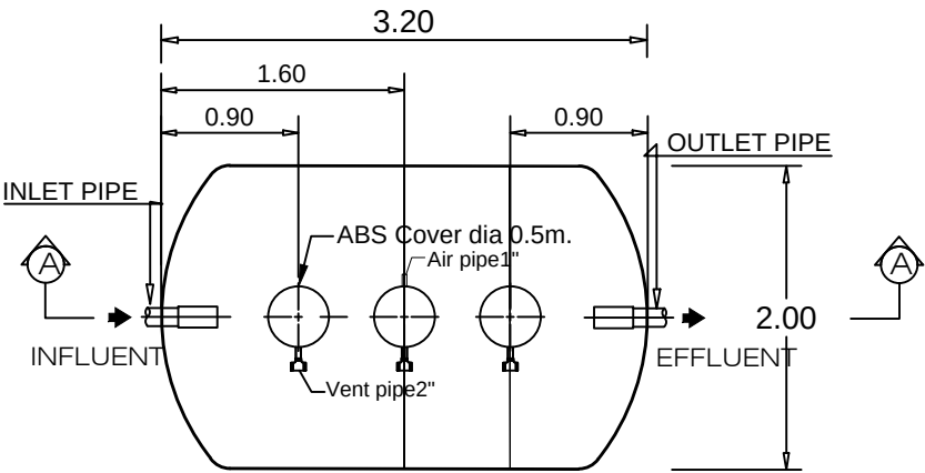
STAR TANK MODEL STD-2010A
