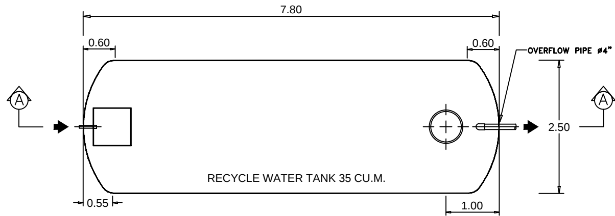
PLAN VIEW SCALE NTS
