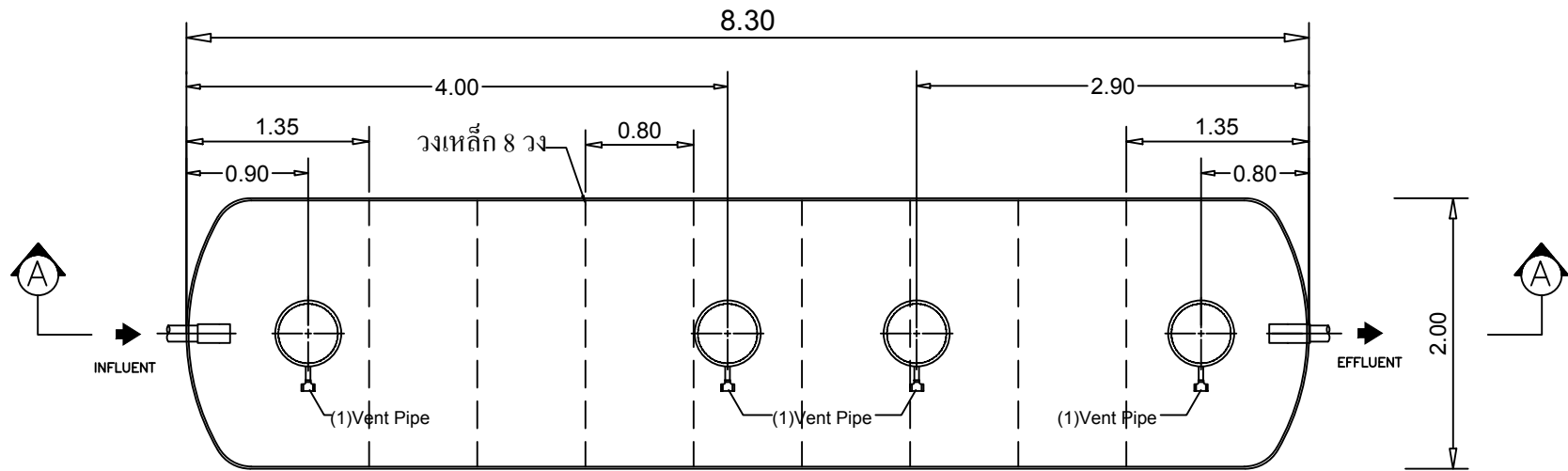
STAR TANK MODEL WSA-2026Z
