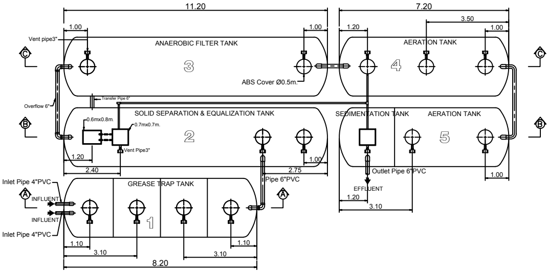
STAR SA-65800Z PLAN VIEW
