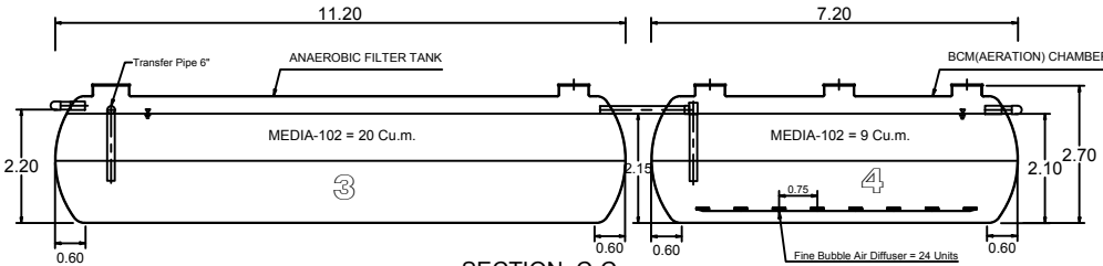
SECTION C-C
