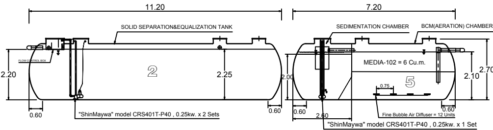
SECTION B-B
