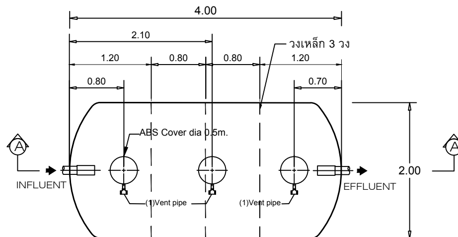
STAR TANK MODEL CFA-12Q
