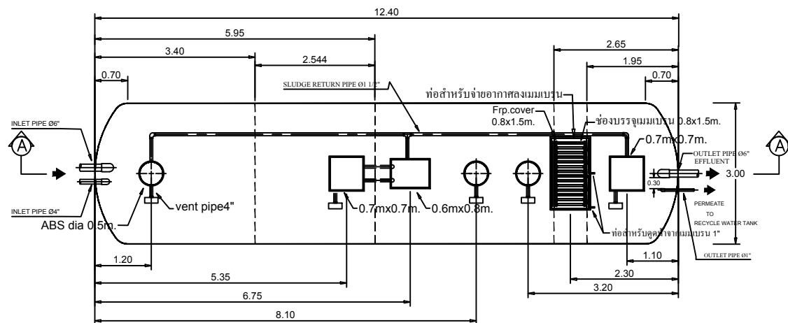
PLAN VIEW / WWT-01
