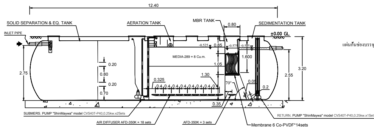
SECTION A-A SCALE MTS
