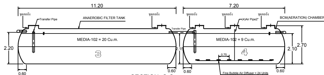
SECTION C-C
