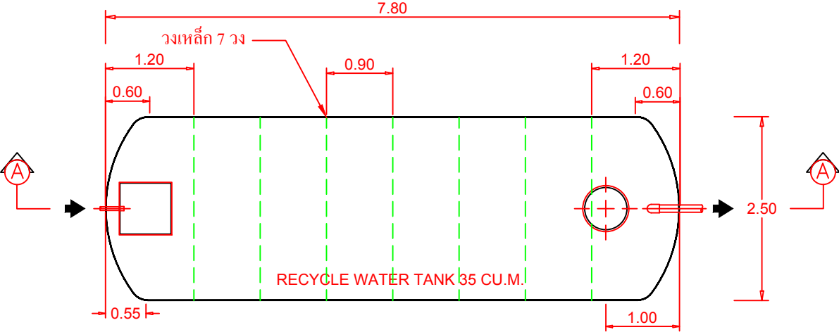
PLAN VIEW SCALE NTS
