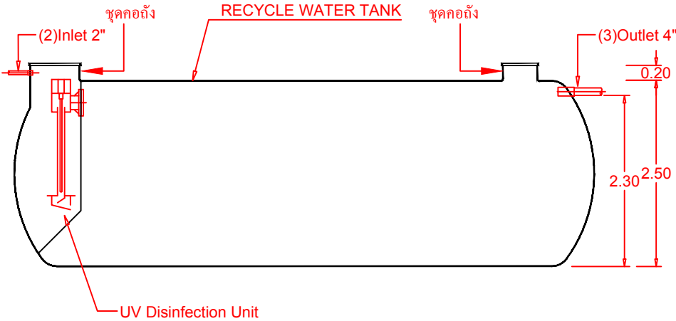
SECTION A-A SCALE NTS
