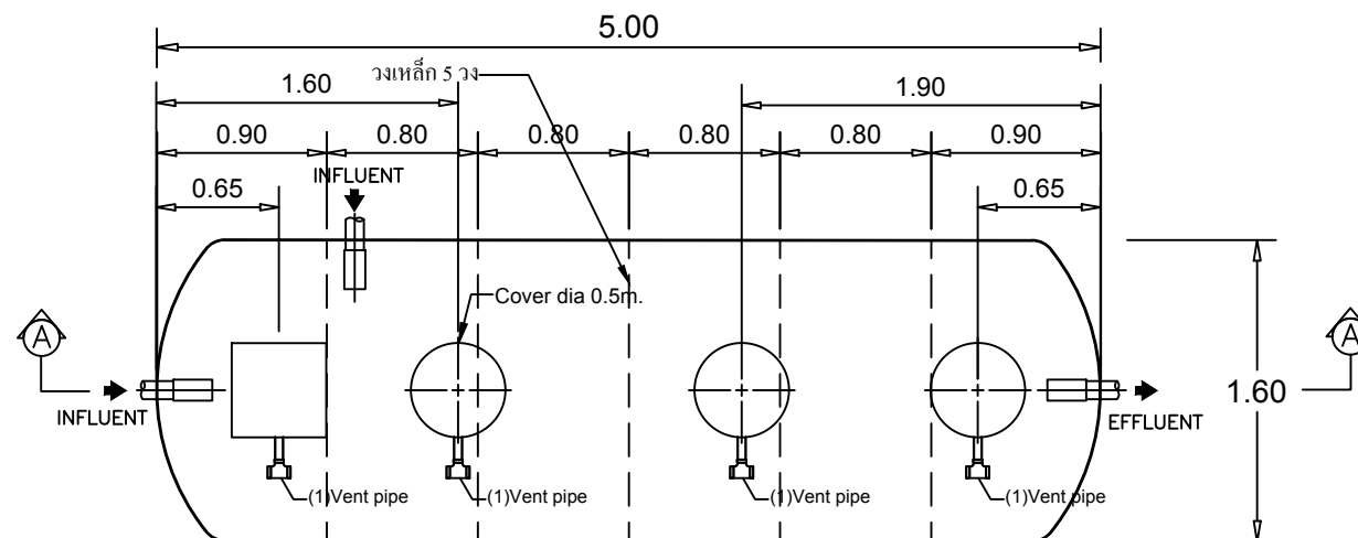
STAR TANK MODEL PRACHA-10
