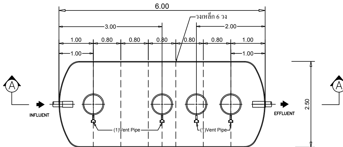
STAR TANK MODEL WSA-2527Z
