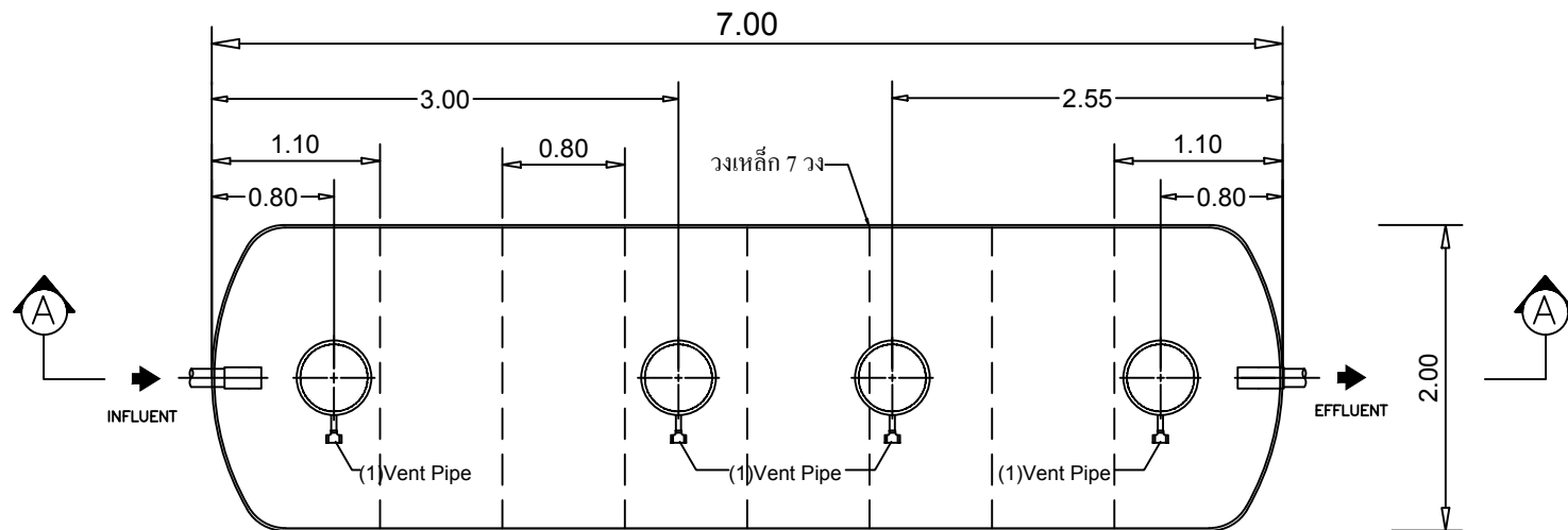
STAR TANK MODEL WSA-2021Z
