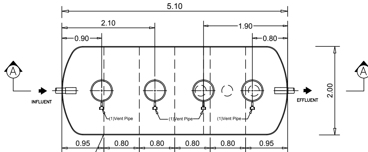
STAR TANK MODEL SSA-2013Z
