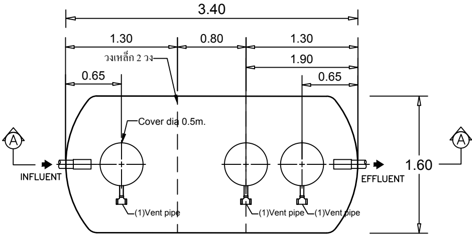
STAR TANK MODEL KWWT-AT6Q
