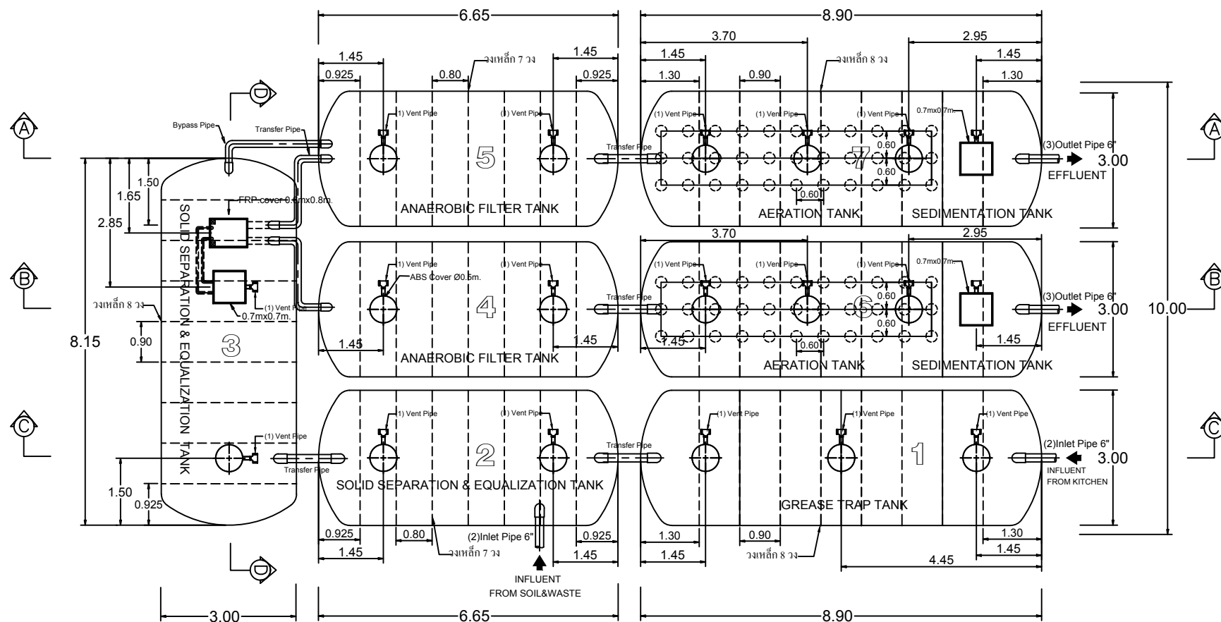
STAR TANK MODEL SA-120800Z PLAN VIEW (ON GROUND)
