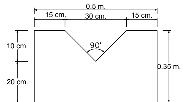
Weir Plate (90°)
