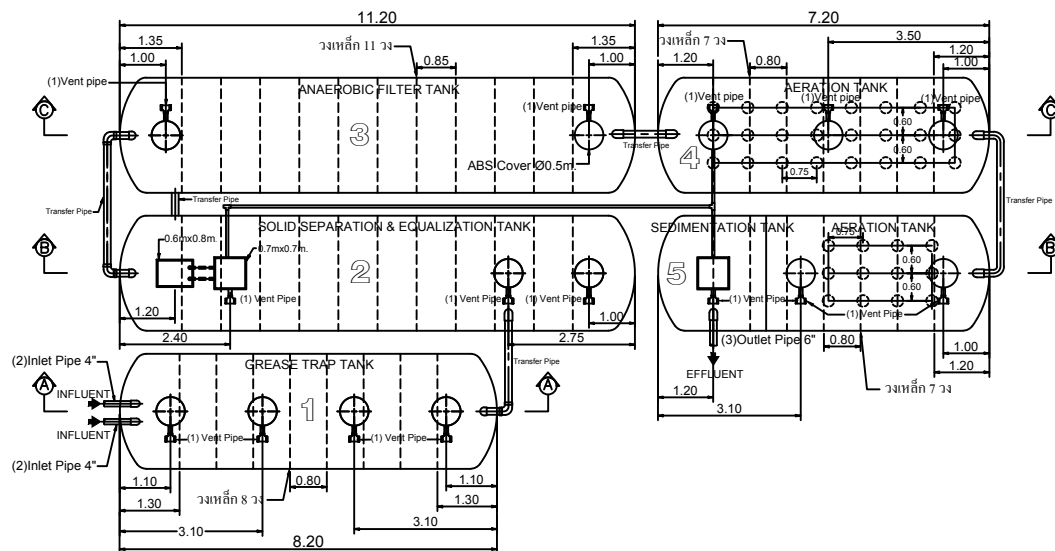
STAR SA-65800Z PLAN VIEW
