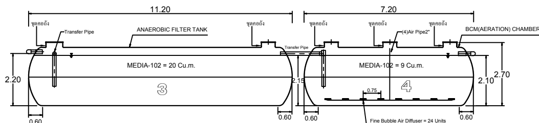
SECTION C-C
