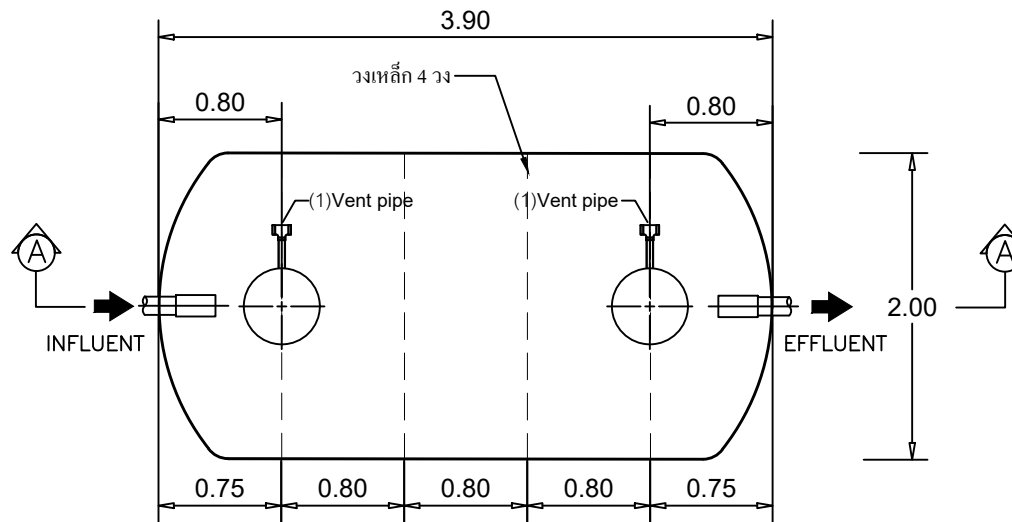
STAR TANK MODEL HSF-10K
