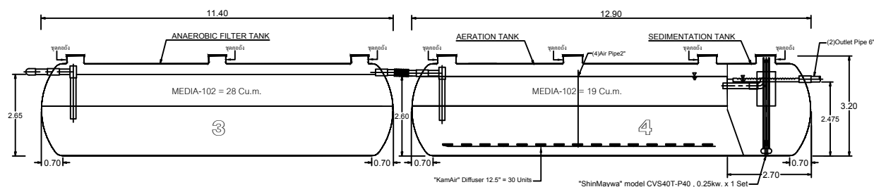
SECTION B-B
