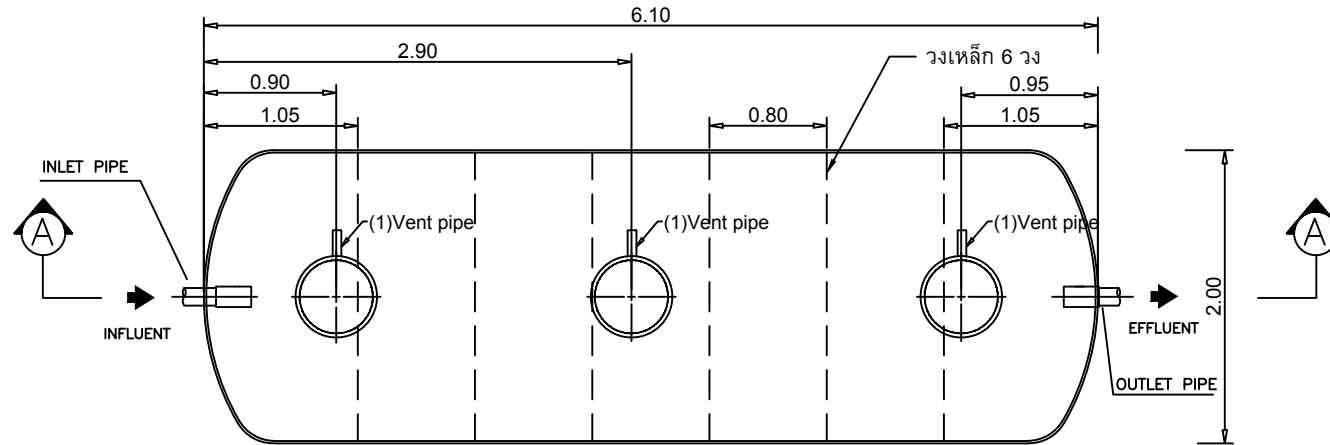
STAR TANK MODEL SS-2016K
