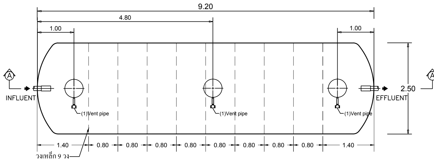
STAR TANK MODEL PT-45FB
