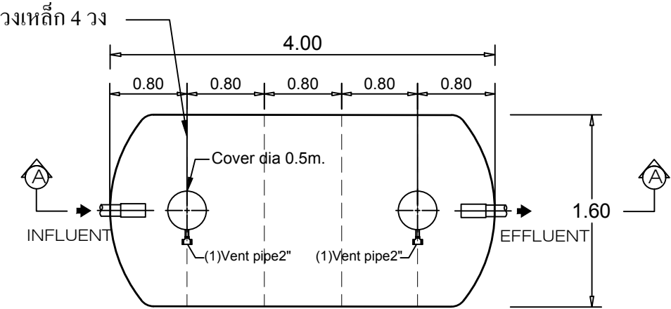
STAR TANK MODEL PS-8
