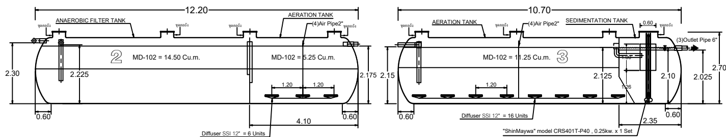
SECTION B-B
