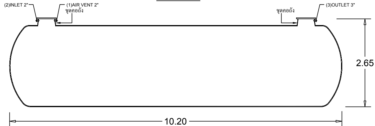
SIDE VIEW
