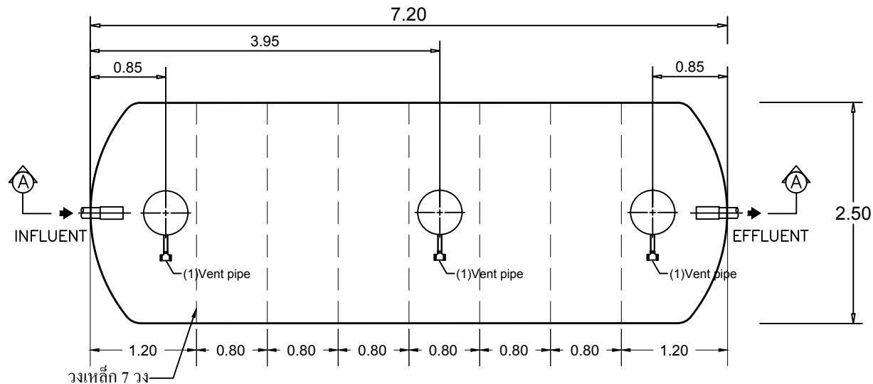
STAR TANK MODEL PSP-35-A
