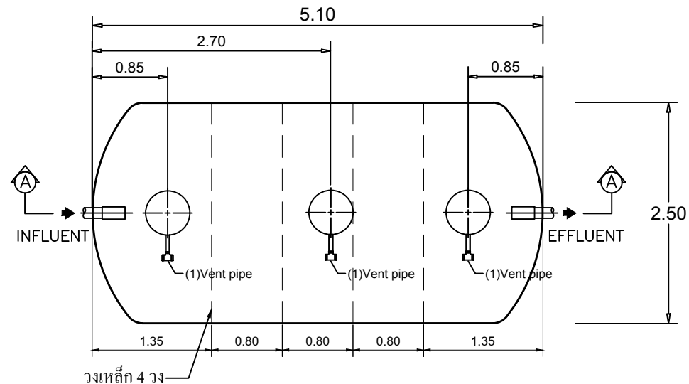
STAR TANK MODEL PSP-25-A
