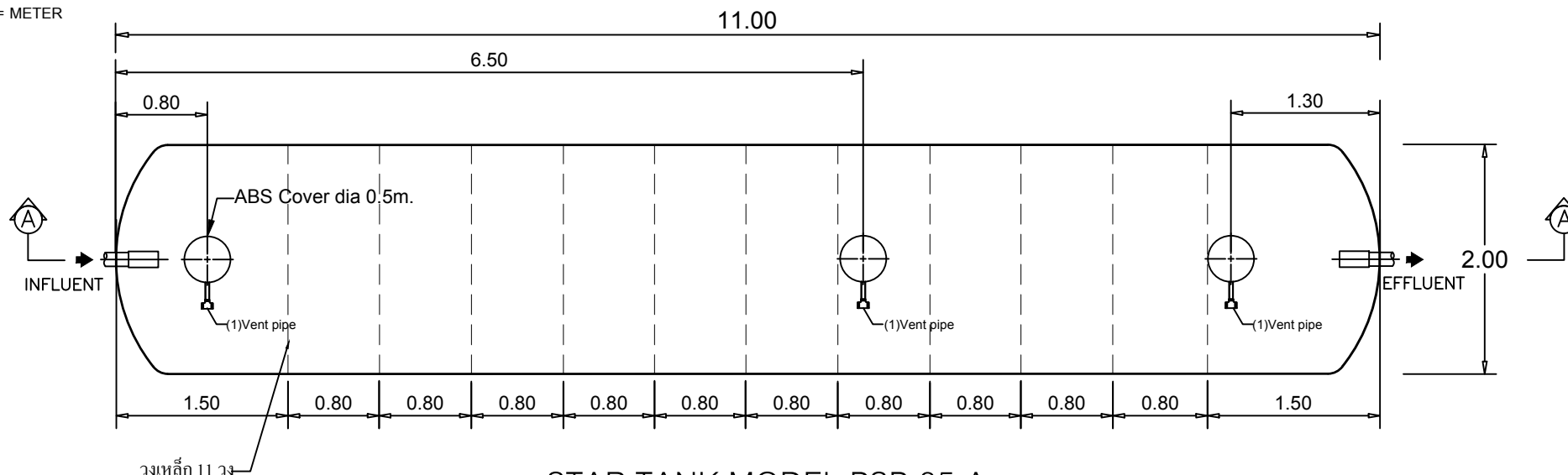
STAR TANK MODEL PSP-35-A
