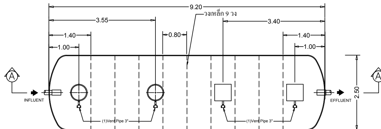
STAR TANK MODEL WSA-2540Z
