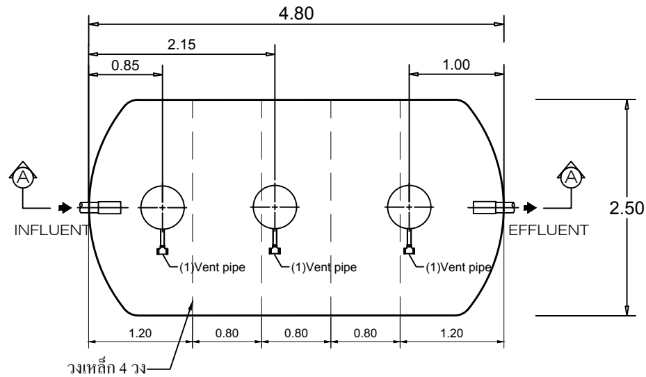
STAR TANK MODEL PT-23(S)
