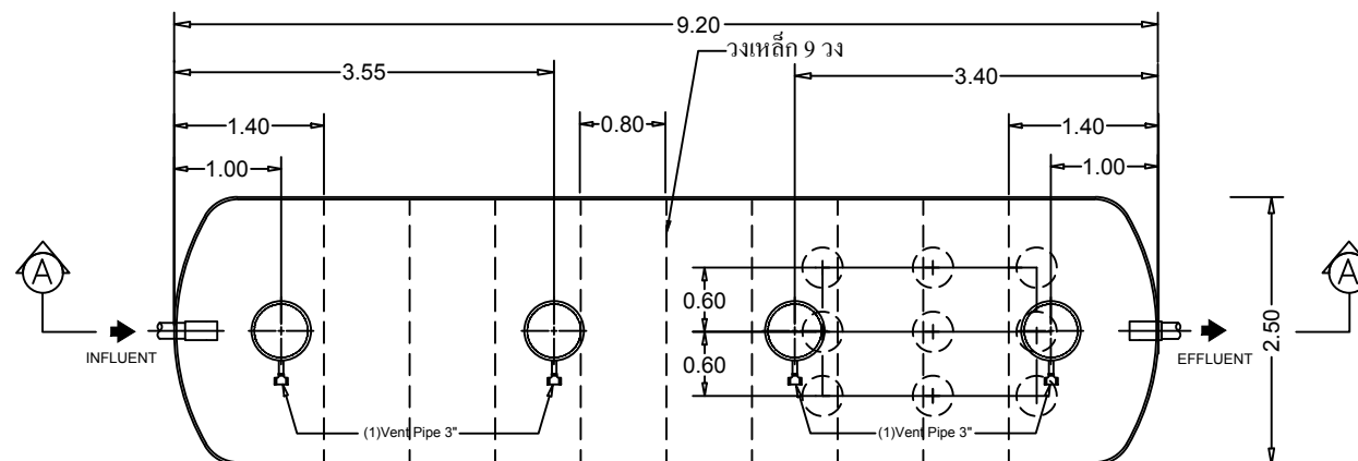
STAR TANK MODEL SSA-2540Z
