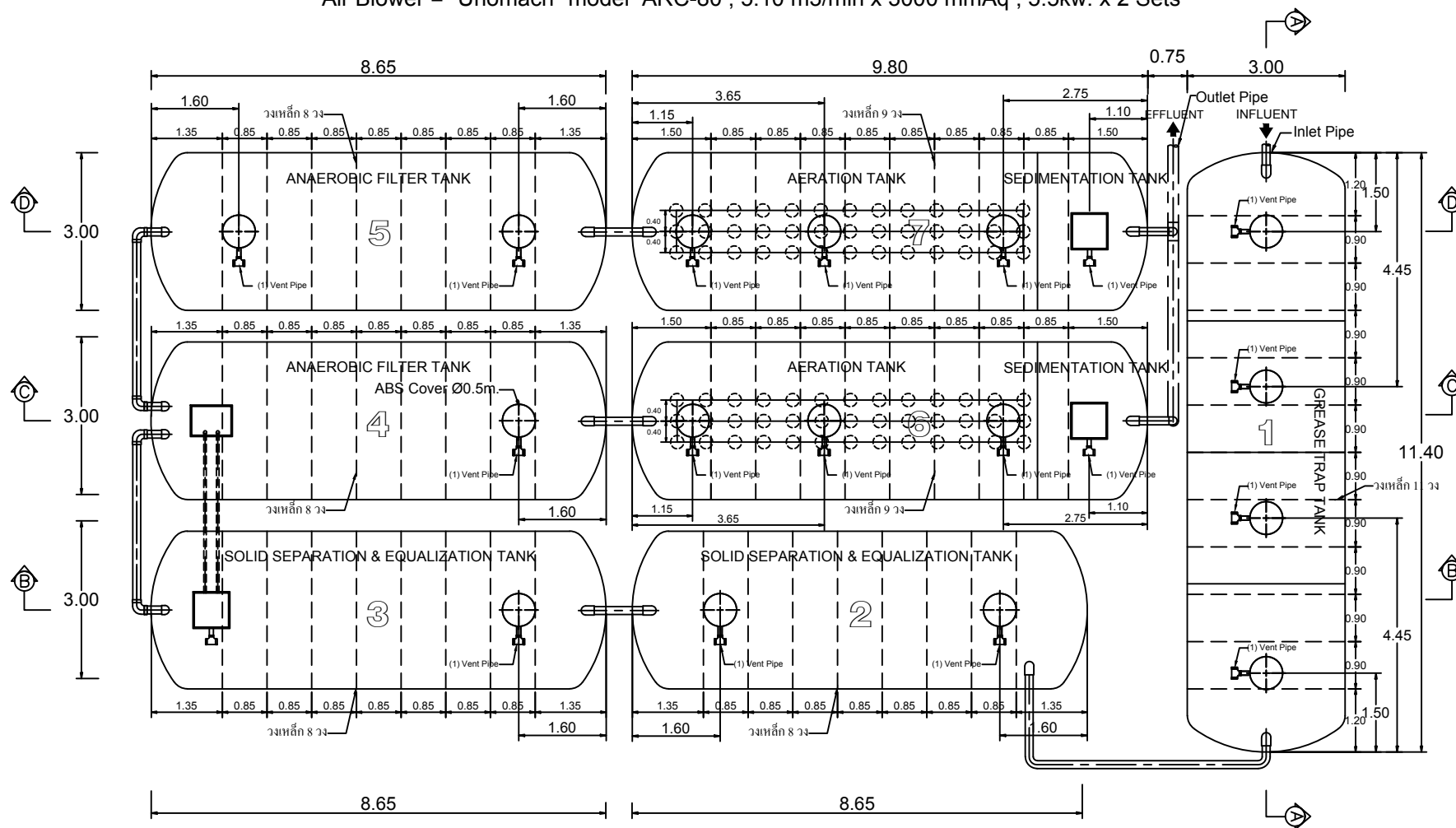
STAR SA-140800Z PLAN VIEW (ON GROUND)
