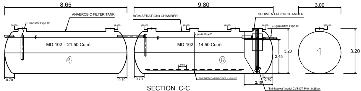
SECTION C-C
