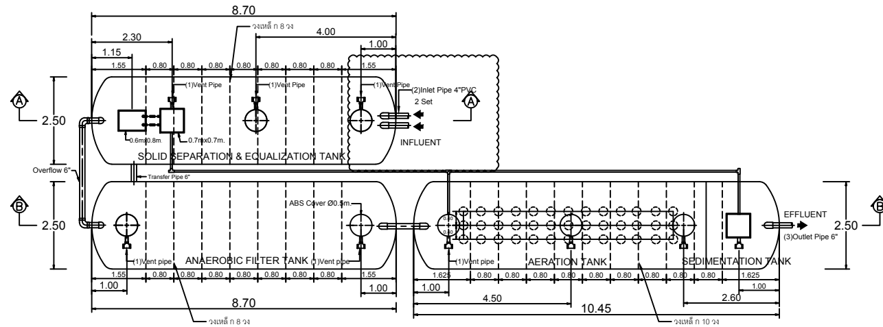
STAR SA-50800Z PLAN VIEW
