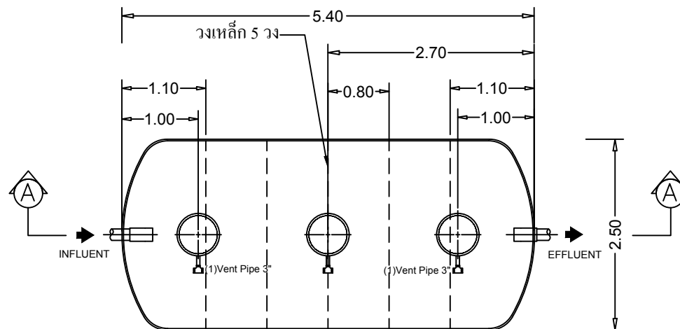
STAR TANK MODEL WS-2525
