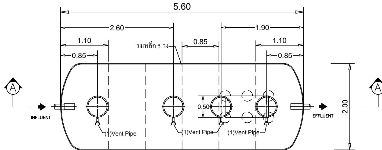
STAR TANK MODEL SS-2015AZ
