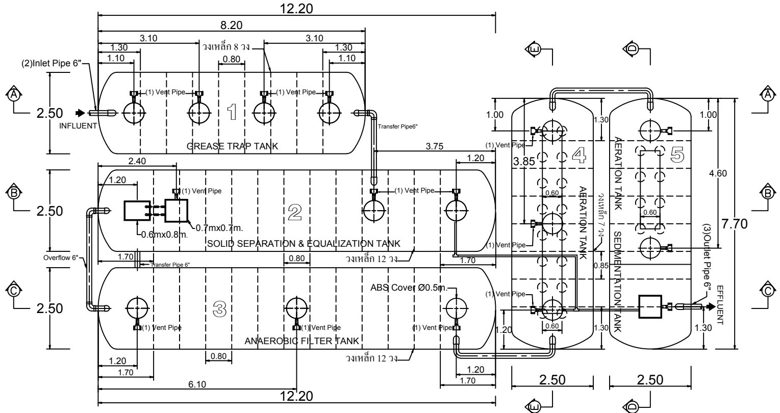
STAR SA-70800Z PLAN VIEW
