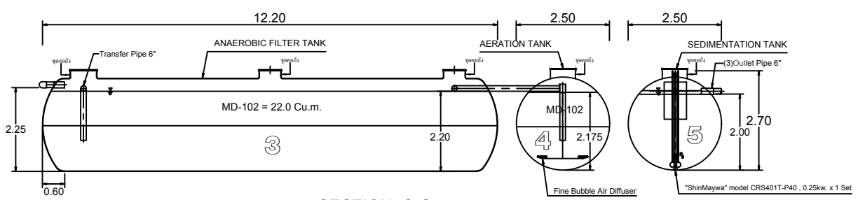
SECTION C-C
