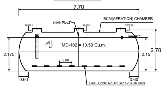
SECTION E-E
