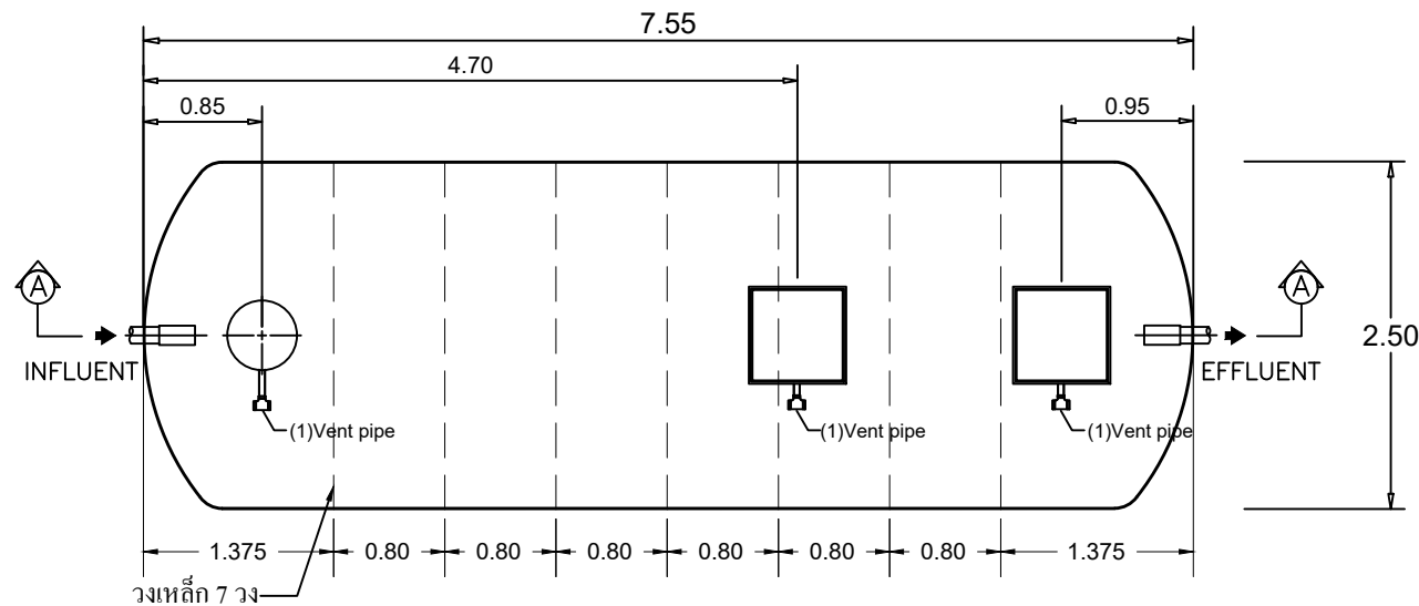
STAR TANK MODEL SP-B90 F100
