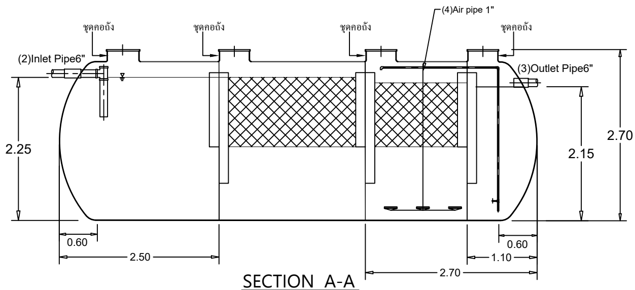
STAR TANK MODEL HEFA-20B
