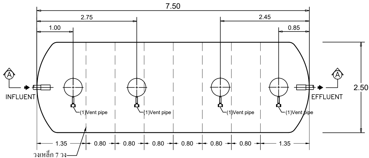
STAR TANK MODEL HEFA-20B
