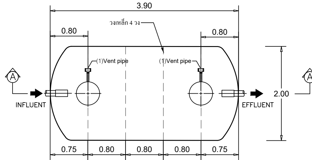
STAR TANK MODEL HSF-10K
