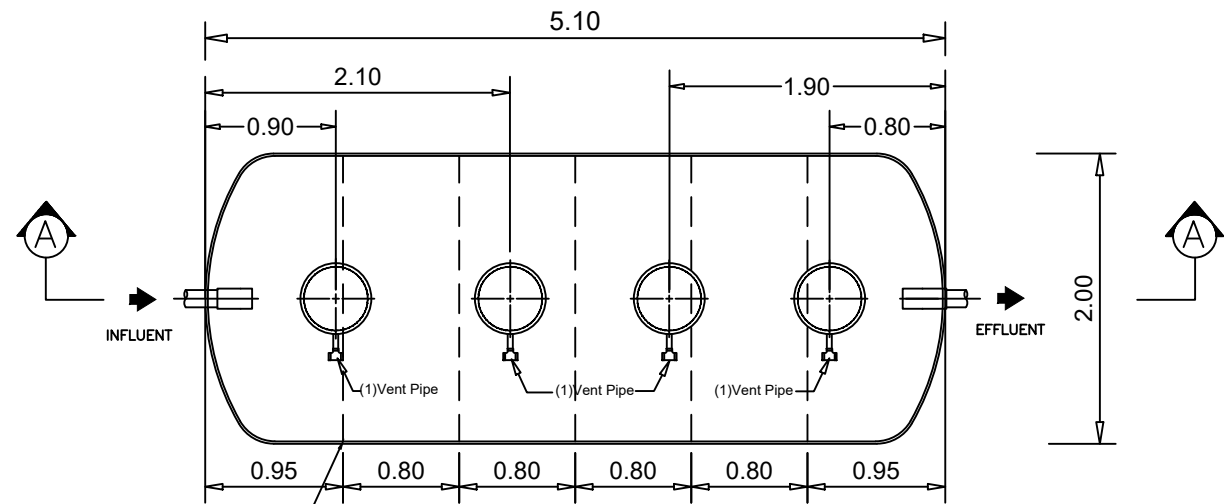
STAR TANK MODEL WSA-2015Z
