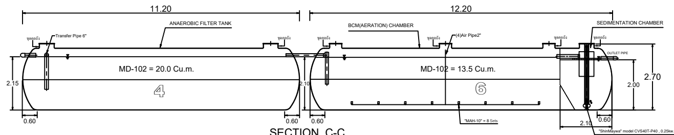
SECTION C-C
