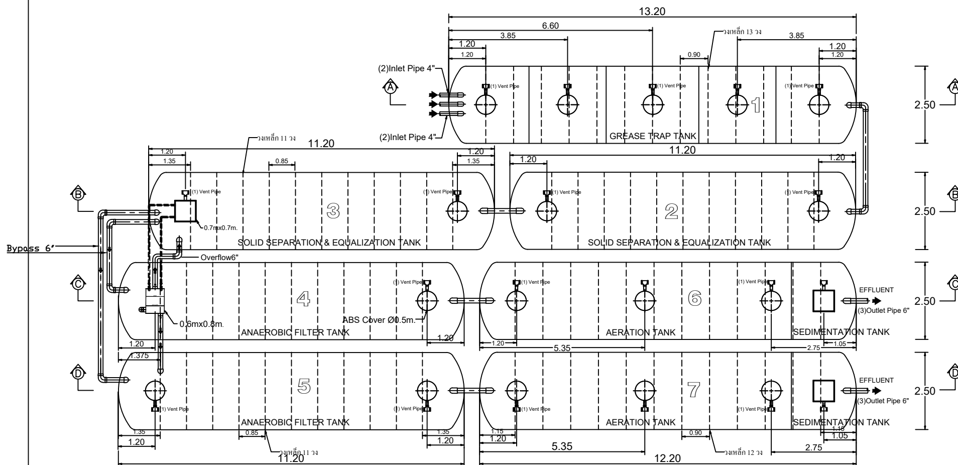
STAR SA-130800Z PLAN VIEW (ON GROUND)
