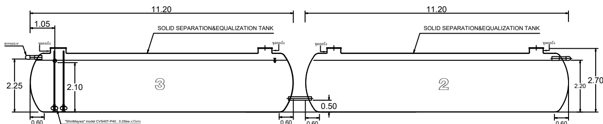
SECTION B-B
