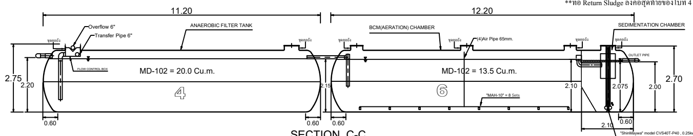
SECTION C-C
