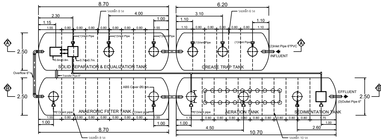
STAR SA-50800Z PLAN VIEW
