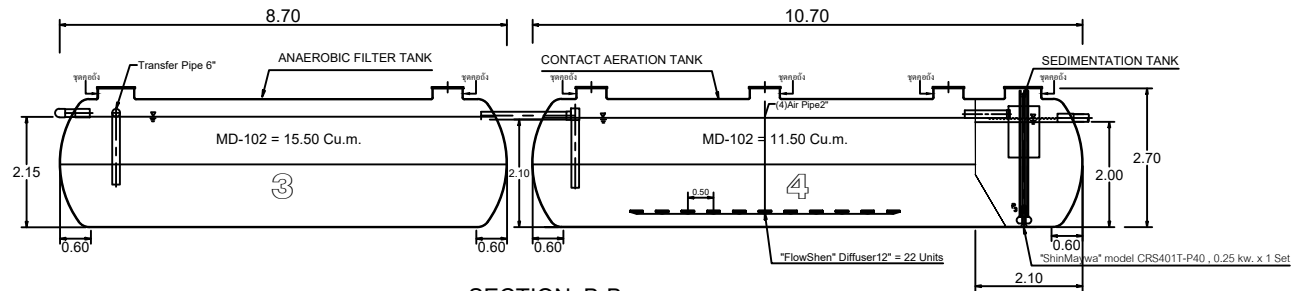
SECTION B-B
