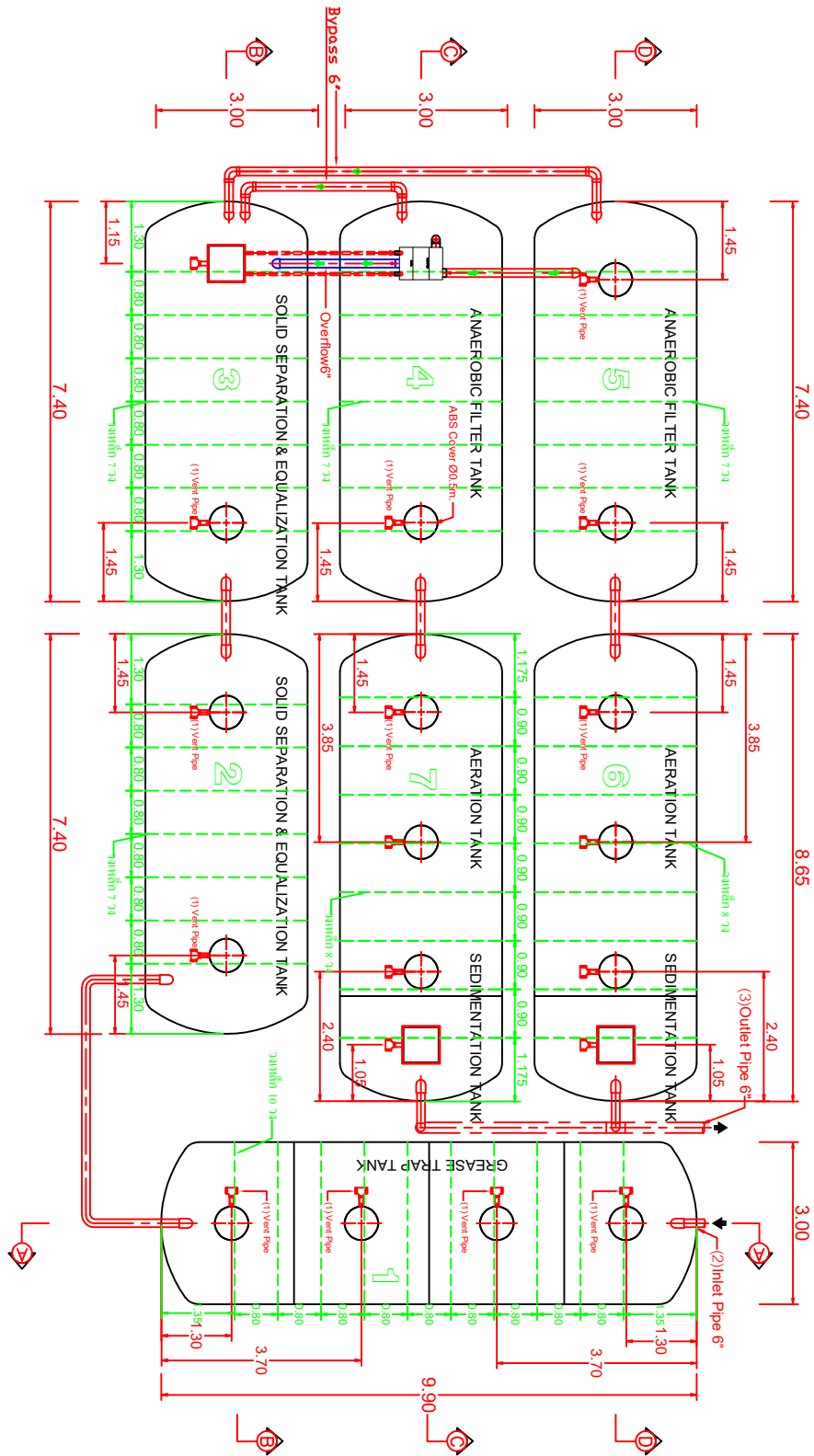
STAR SA-120800ZD3 PLAN VIEW
