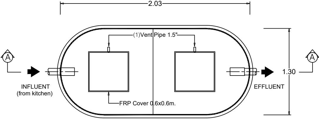
PLAN VIEW
